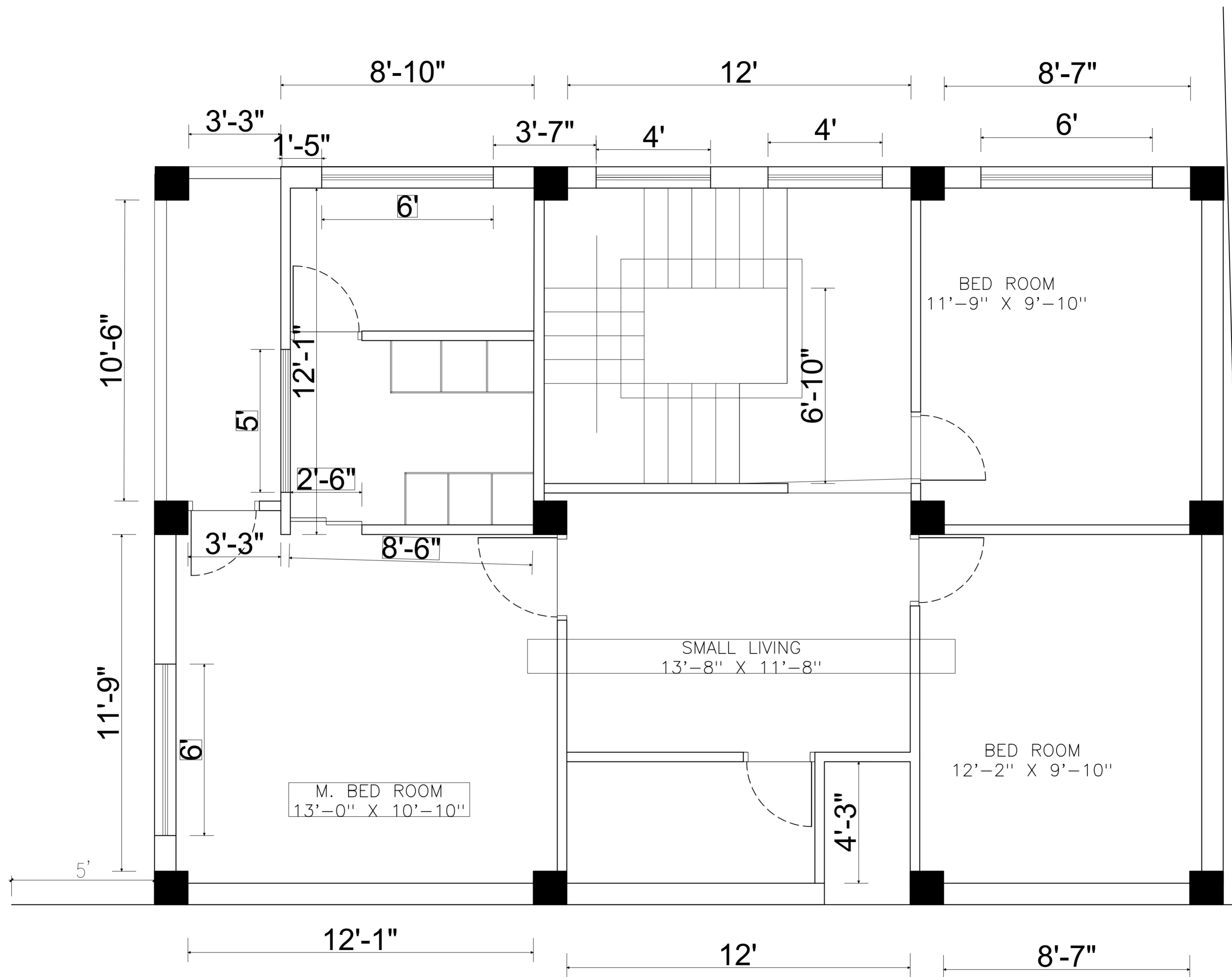
SECOND FLOOR PLAN SECOND FLOOR AREA:- 955.00 SQ.FT TOTAL AREA:-1372.00 SQ.FT.
